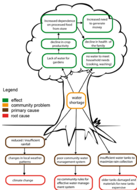
Figure 33: Problem tree 31
